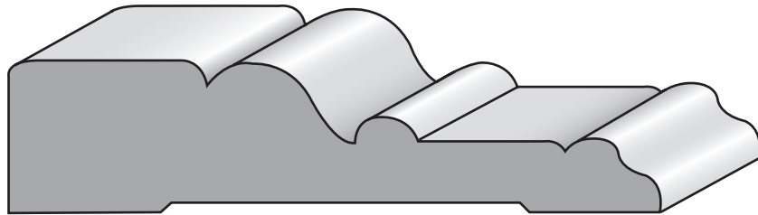
PAC 6123 7/8 X 3-3/4
