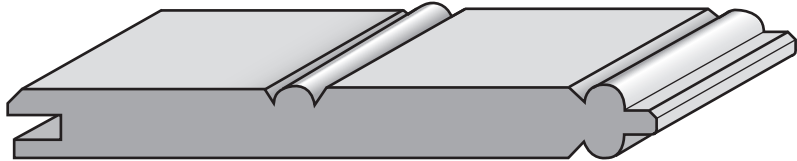
PAC 8510 3/8 X 3-3/8 (3-1/4" Face)
