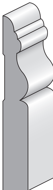
PAC 2115 9/16 X 3-7/8
