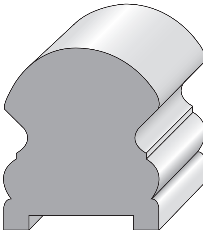
PAC 4112 2-5/8 X 3
