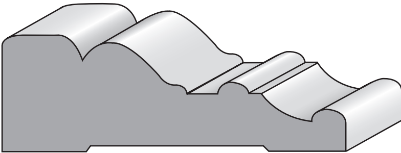
PAC 6124 1-3/16 X 3-1/2
