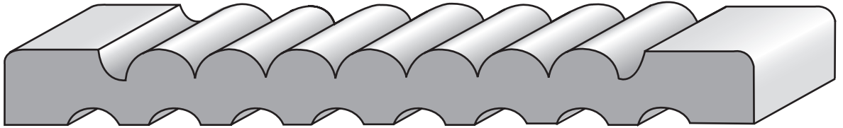
PAC 6125 9/16 X 5-1/2 Reversible
