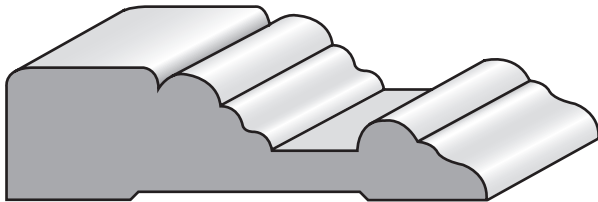
PAC 6137 11/16 X 2-1/2
